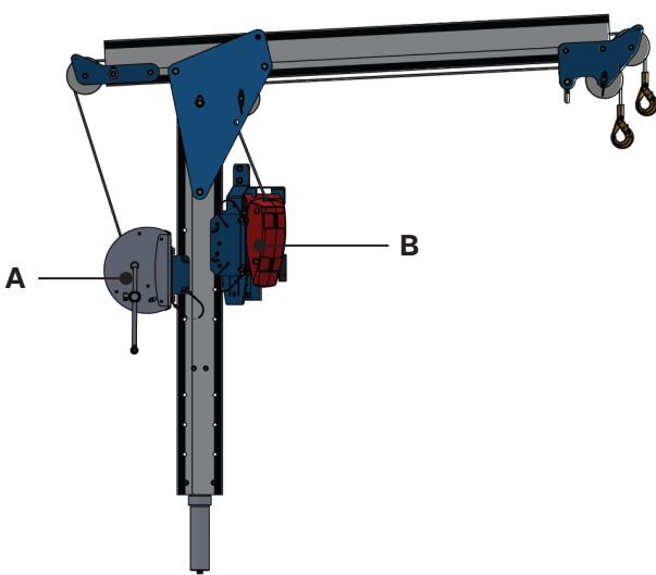
T DAVIT DOUBLE WINCHED
