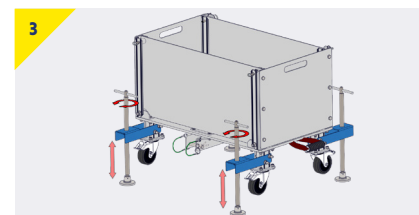
Operate the Height Adjustable Feet to the required height
